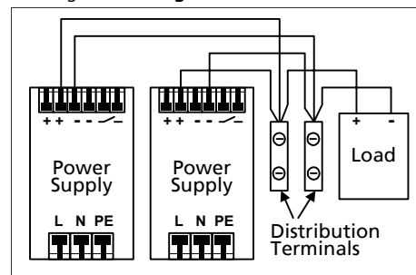
Fig. 27-7 Using distribution terminals
